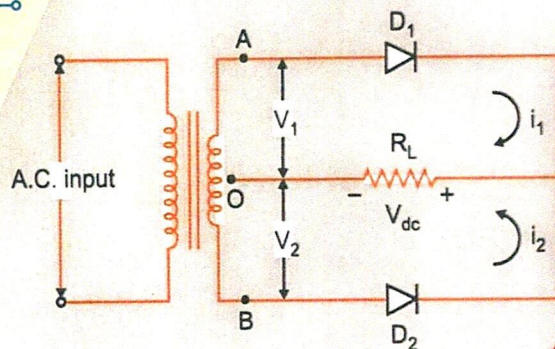
Full-wave rectifier
