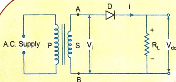
Half-wave rectifier
