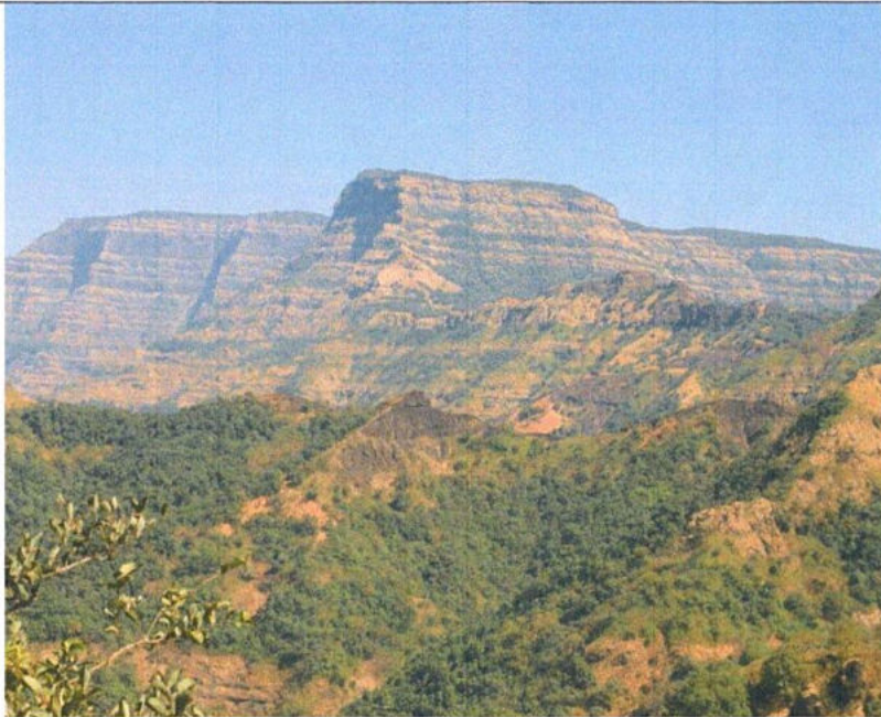
Plate 1: Basaltic Lava Flows
