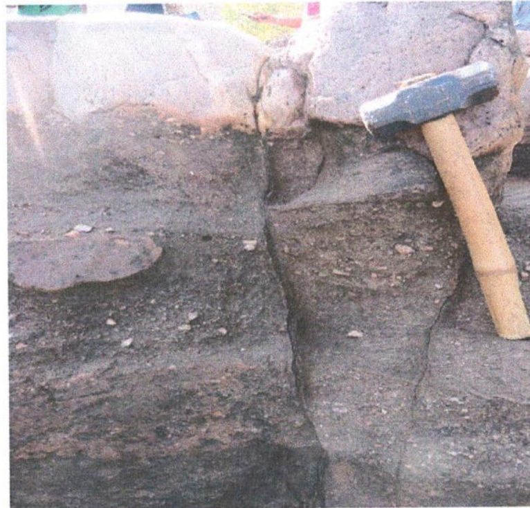
(Plate 8): Eparchean Unconformity near Shravan, Dist. Sindhudurg.
