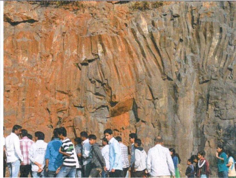
(Plate 4): Columnar Joints of Mahad
