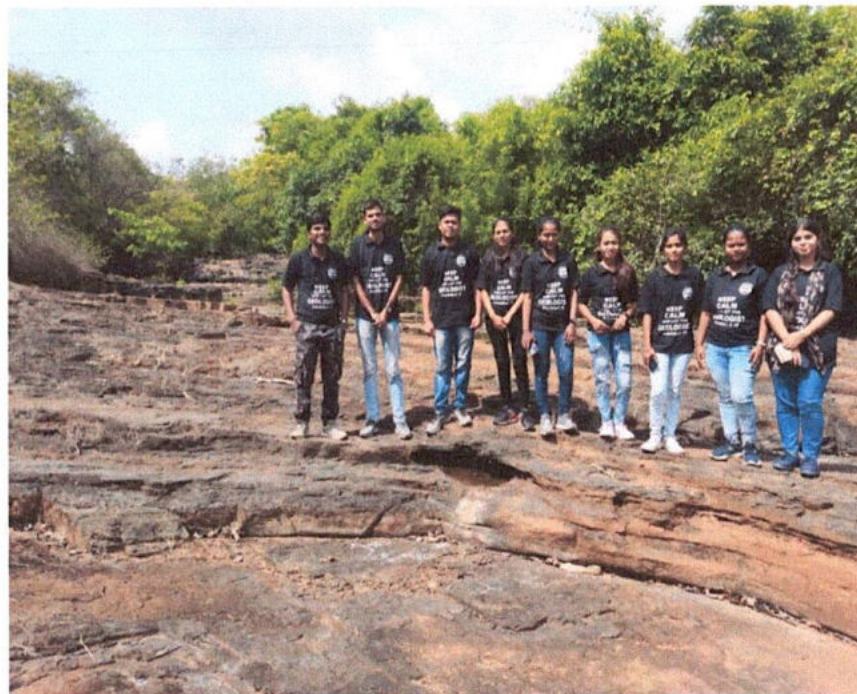
(Plate 2): Slates of Chunakolvan, Dist. Ratnagiri.
